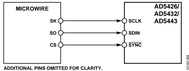
Figure 57. MICROWIRE-to-AD5426/AD5432/AD5443 Interface PIC16C6x/7x to AD5426/AD5432/AD5443
