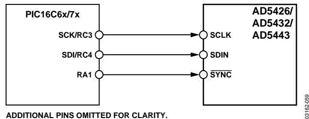
Figure 58. PIC16C6x/7x-to-AD5426/AD5432/AD5443 Interface
