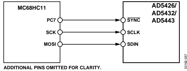
Figure 56. 68HC11/68L11-to-AD5426/AD5432/AD5443 Interface MICROWIRE to AD5426/AD5432/AD5443 Interface
