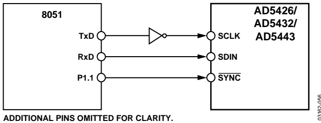
Figure 55. 80C51/80L51-to-AD5426/AD5432/AD5443 Interface
